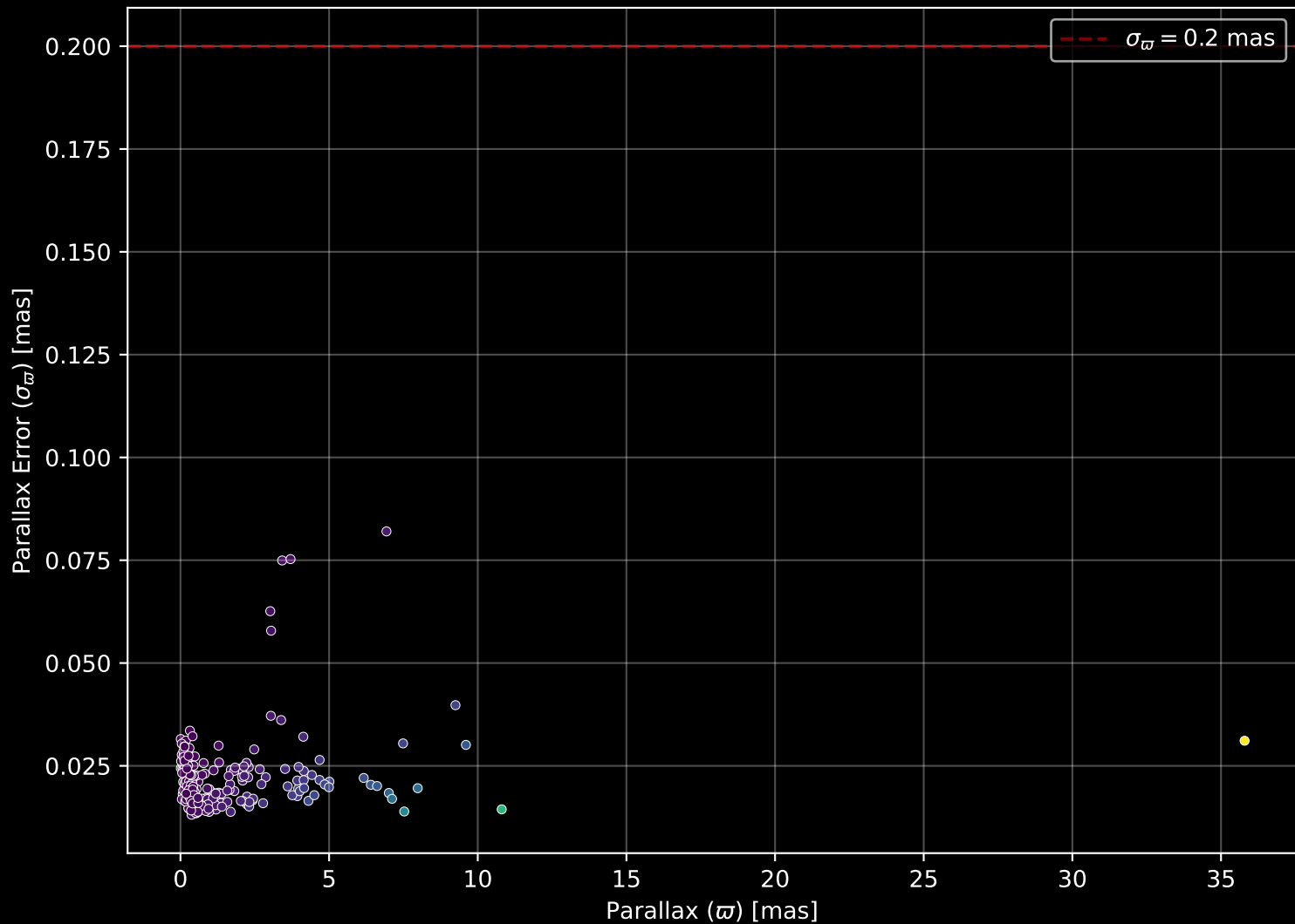
APOGEE DR17 Field: [266+44] Parallax Quality (n= 201)
